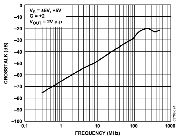
Figure 37. Large Signal All-Hostile Crosstalk
