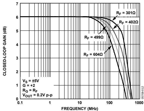
Figure 10. Small Signal Frequency Response vs. R_F
