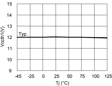
Figure 13. V CC UV turn-on threshold vs. temperature
