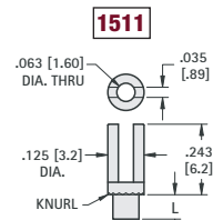
Staking Tool No. TL-3
