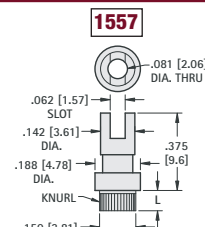
Staking Tool 1557-TL
