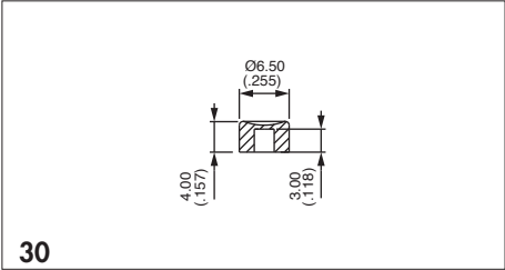
P/N U4310 - for long plunger only
