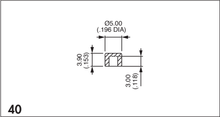
P/N U4320 - for long plunger only
