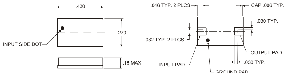
Outline Drawing
