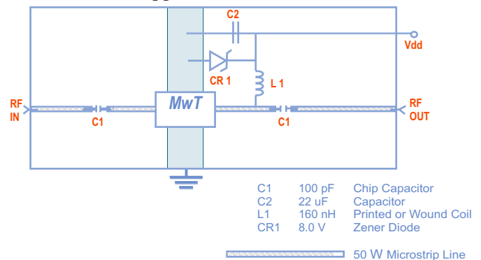
Application Circuit
