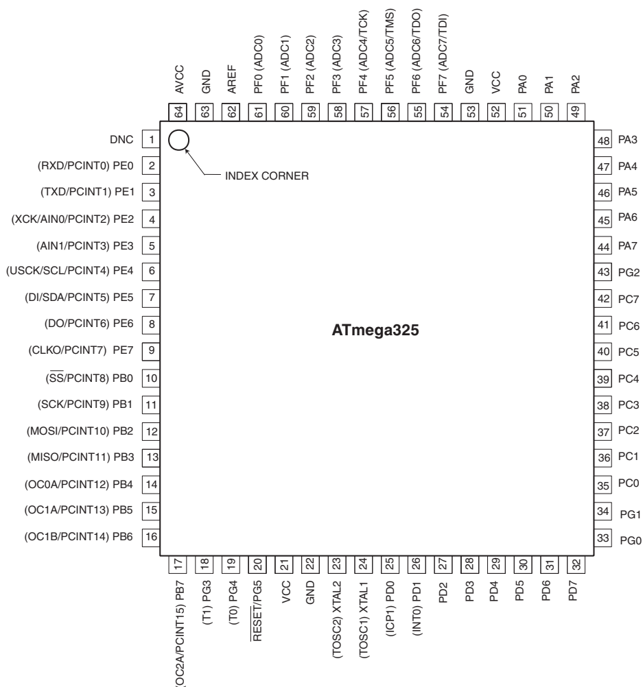
Figure 1-2. Pinout ATmega325P
