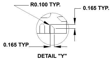
DETAIL "Y"
