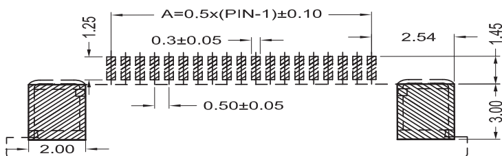
R3 and R4 PCB Layout Reference
