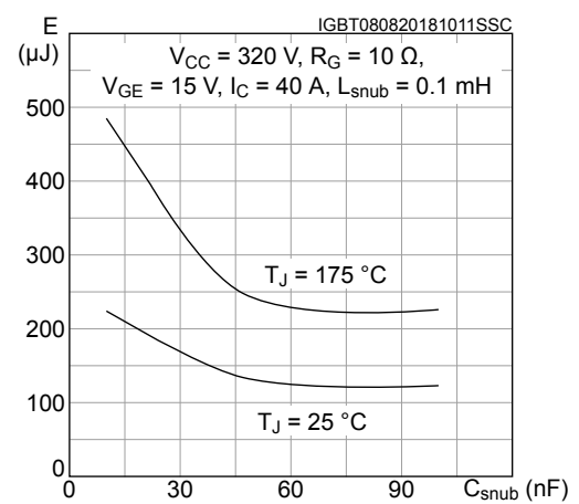
Figure 18. Switching energy vs snubber capacitance
