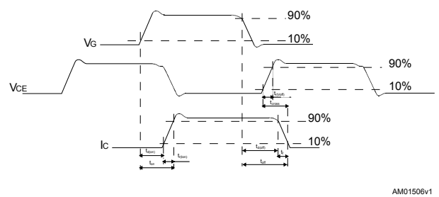
Figure 24. Switching waveform
