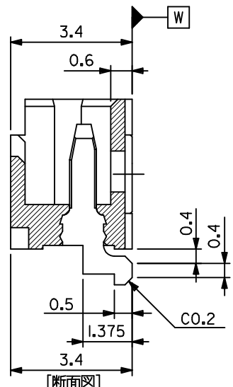
[断面図]
