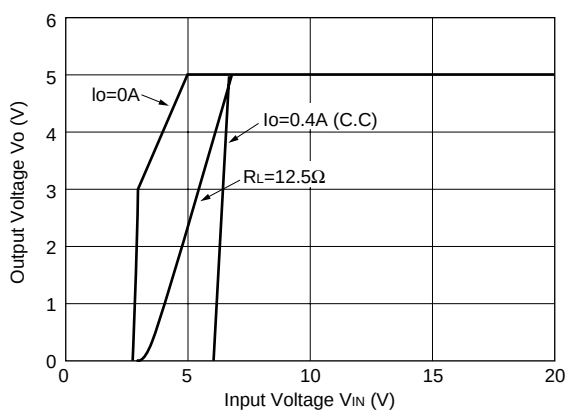
Rise Characteristics
