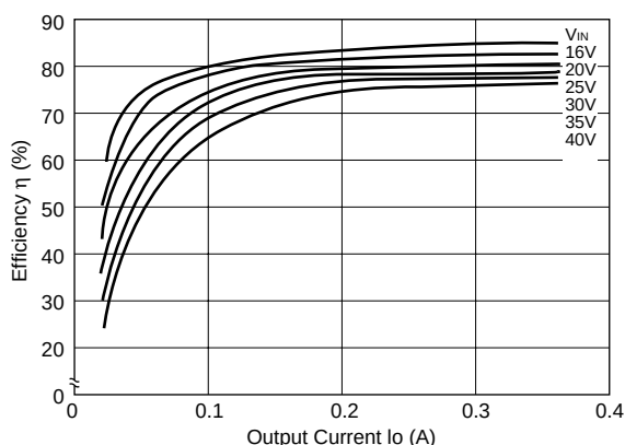
Efficiency Characteristics
