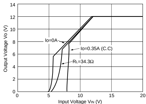
Rise Characteristics
