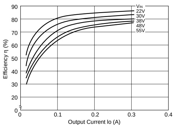
Efficiency Characteristics
