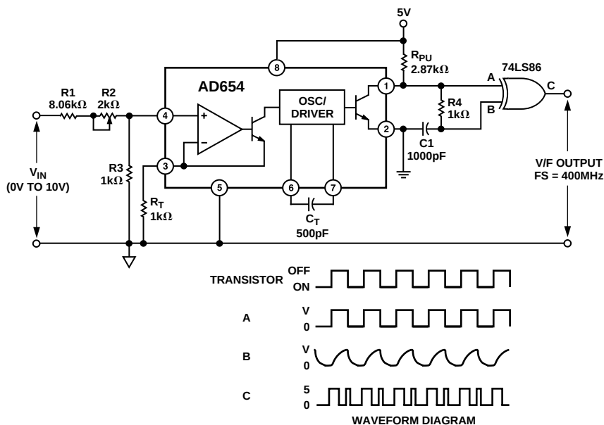
Figure 11. AD654 VFC as an ADC
