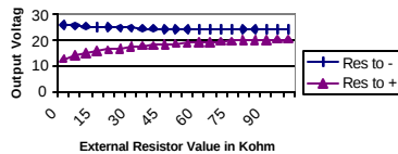
PM3048D12 Voltage Trim Adjusts the total voltage (+) out to (-) out
