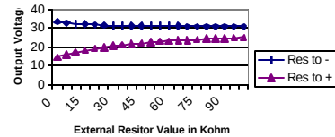
PM3048D15 Voltage Trim Adjusts the total voltage (+) out to (-) out
