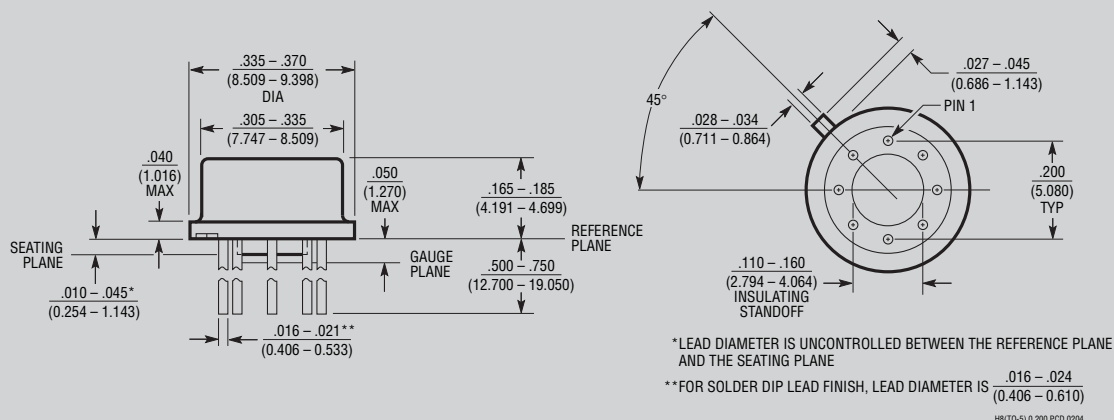
J8 Package 8-Lead Cerdip (Narrow .300 Inch, Hermetic) (Reference LTC DWG # 05-08-1110)
