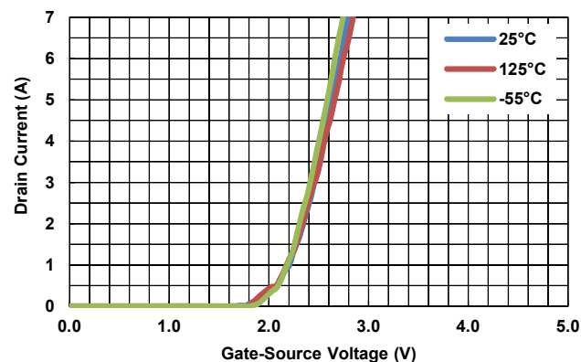
Figure 6. Transfer Characteristics
