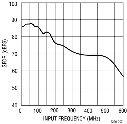
LTC2220: SFDR (HD2 and HD3) vs Input Frequency, -1dB, 1V Range, LVDS Mode
