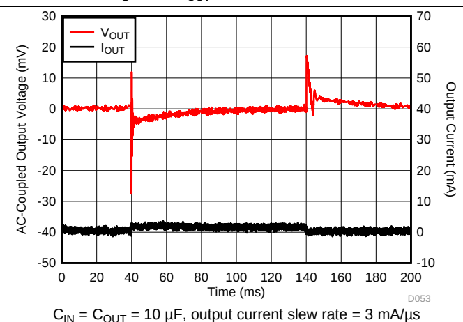
Figure 16. I_{OUT} Transient 3 μA to 3 mA
