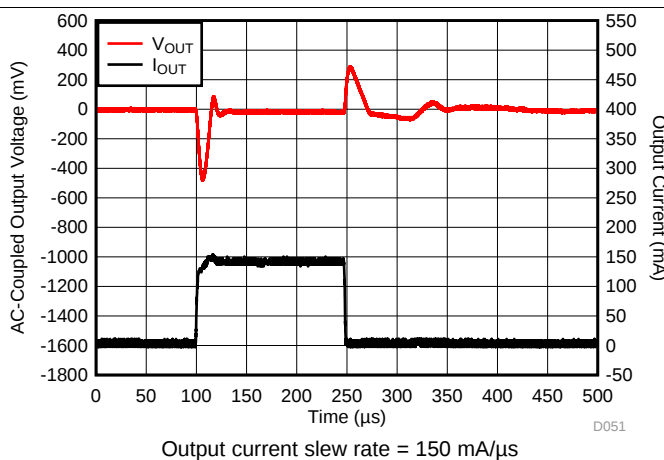
Figure 14. I_{OUT} Transient 1 mA to 150 mA
