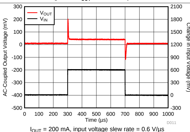
Figure 18. V_{IN} Transient
