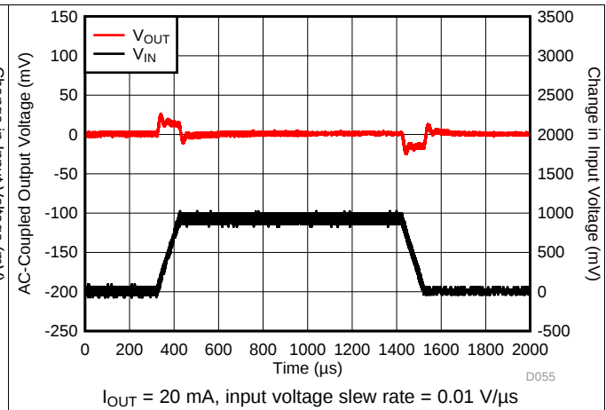
Figure 20. V_{IN} Transient
