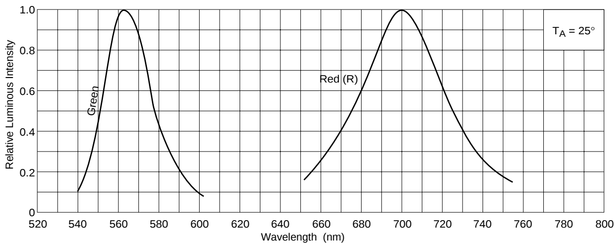
Relative Luminous Intensity vs. Wavelength
