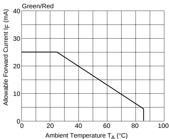
I_V vs. T_A
