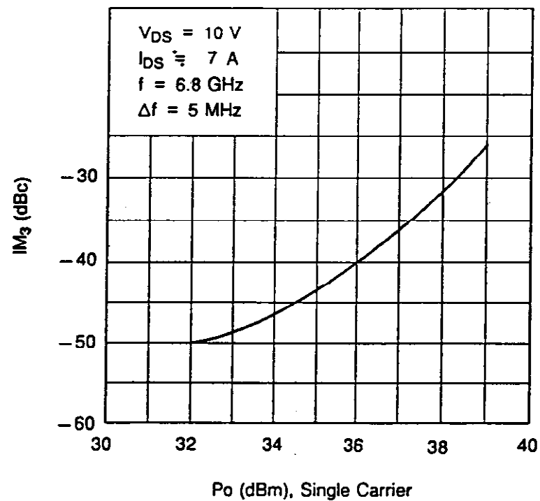
\text{IM}_3 vs. Output Power Characteristics
