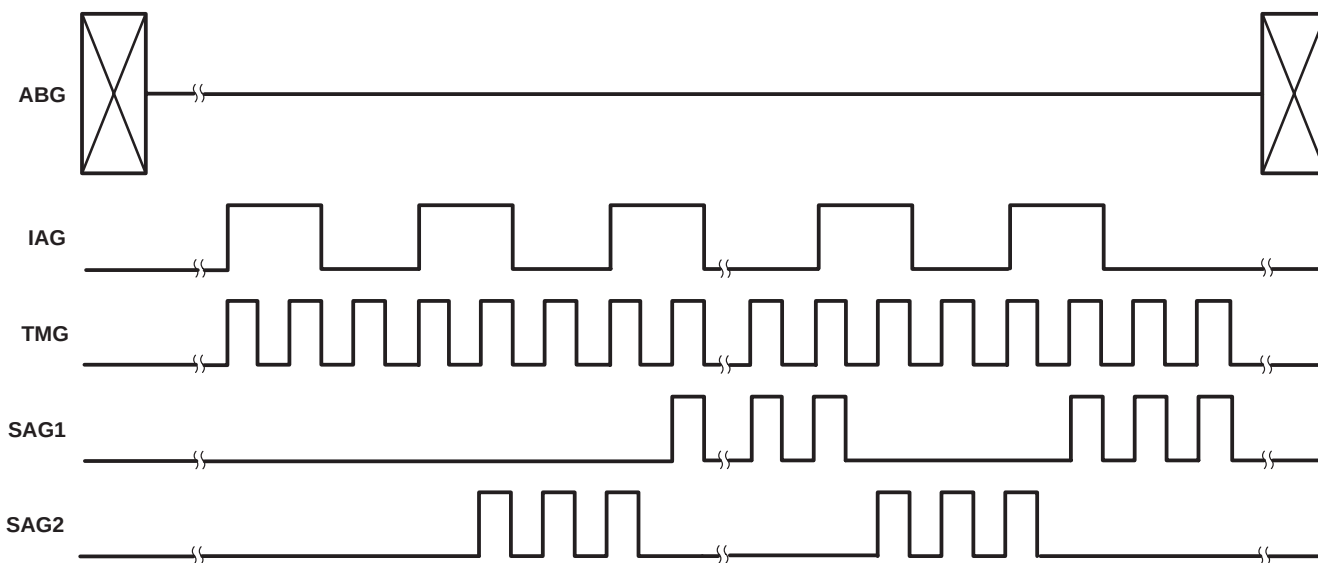
Figure 10. Parallel-Transfer Timing
