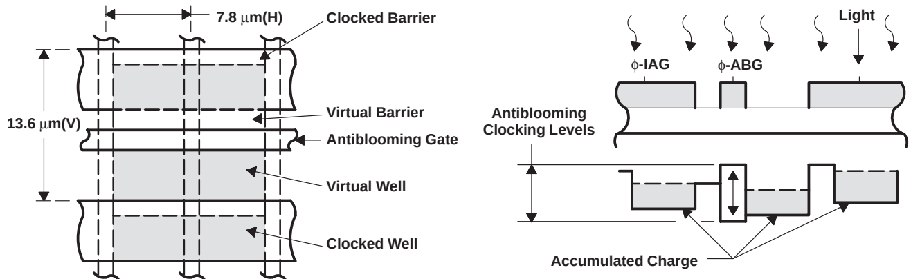
Figure 1. Charge-Accumulation Process
