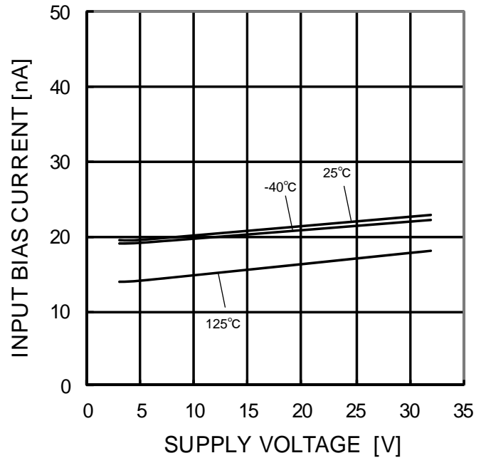
Figure 15. Input Bias Current – Supply Voltage ( V_{icm}=0V , OUT=1.4V )
