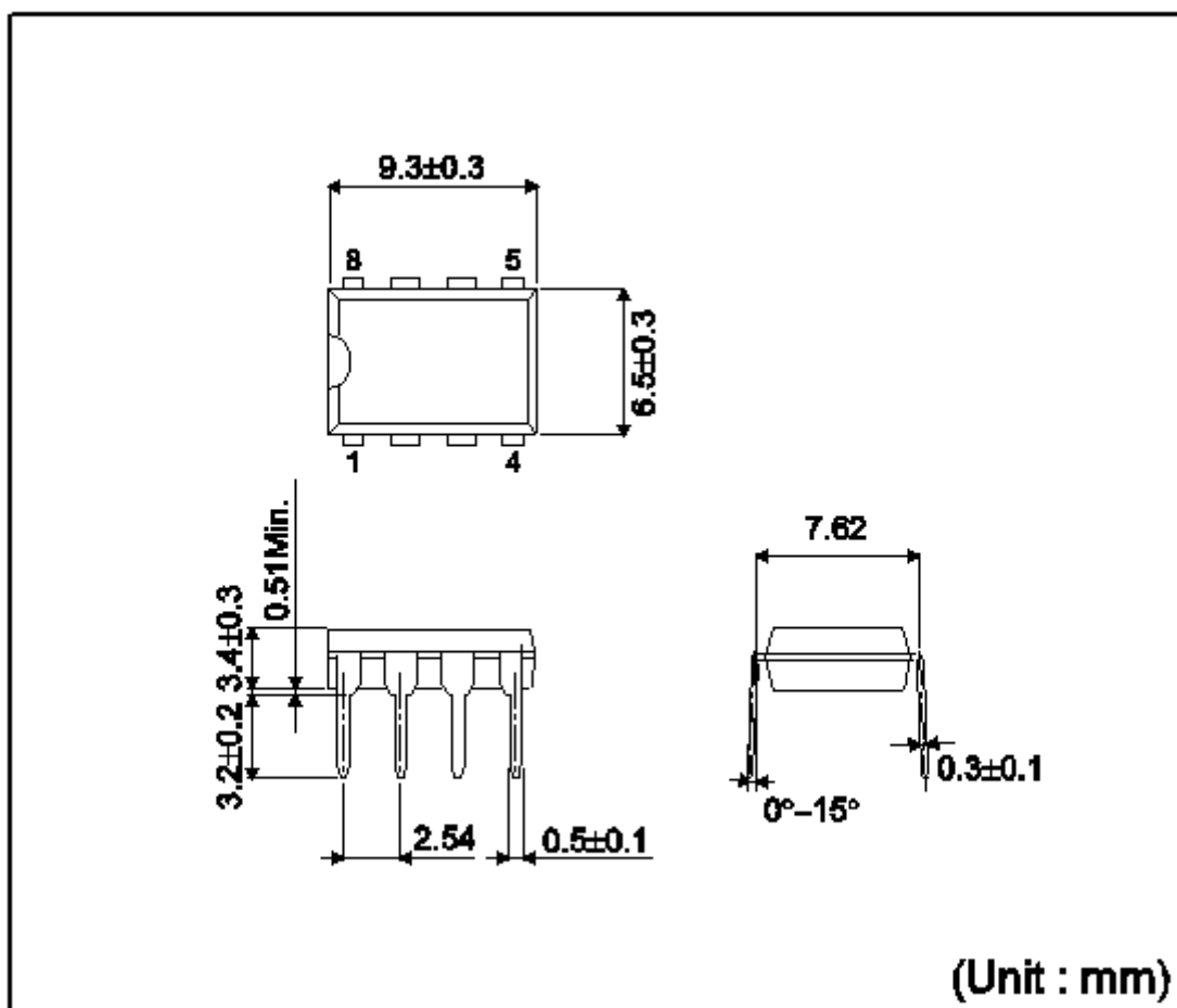
DIP-T8
