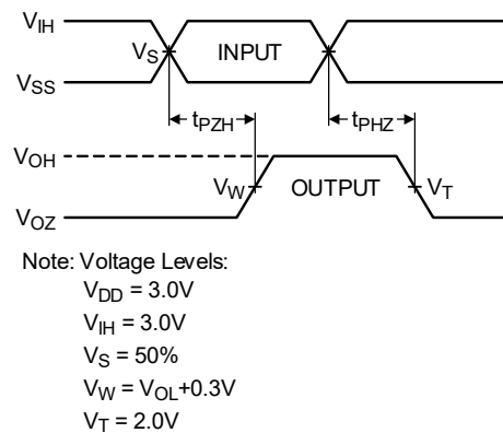
Figure 7. Tri-State High Timing Diagram
