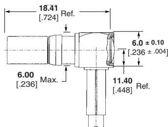
Part Number 148342-1
