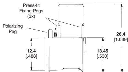
End View of Type M-MSK
