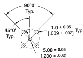
Part Number 148385-1 Recommended PC Board Layout
