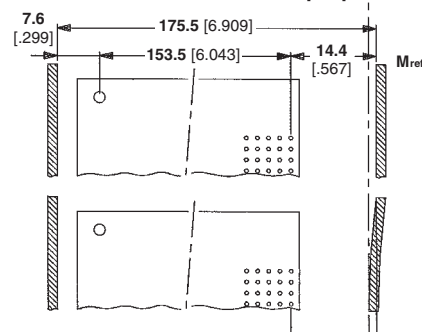
Subrack tolerances
