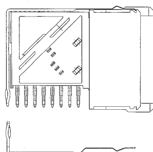
With Shields
