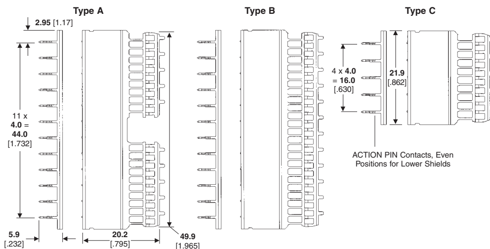
Lower Shields
