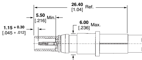
Part Number 148338-4
