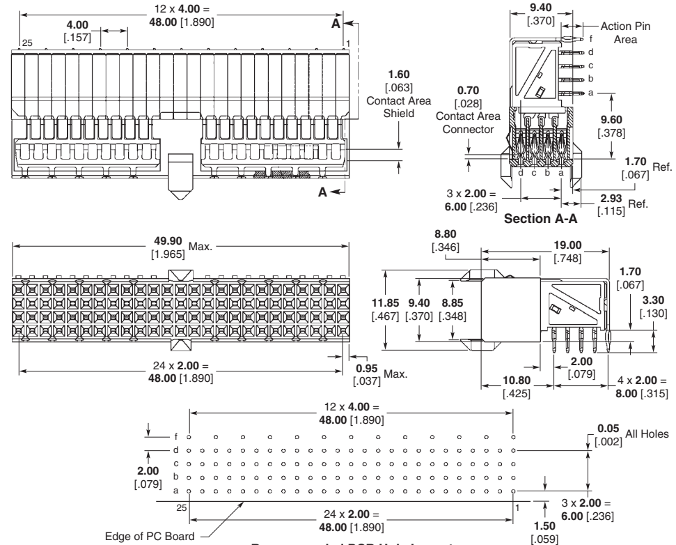
Recommended PCB Hole Layout Component Side Shown
