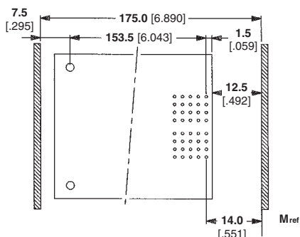
Coordination Dimensions
