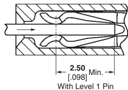
Contact Range
