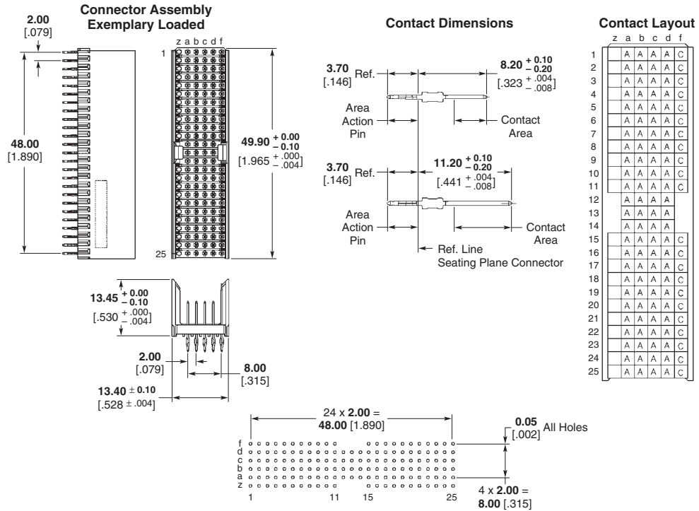
Recommended PCB Hole Layout Component Side Shown
