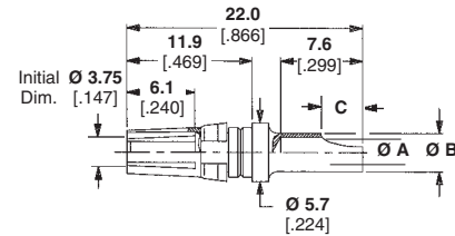
Female, Cable
