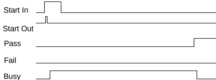
Figure 3-3. Tester I/O Signals
