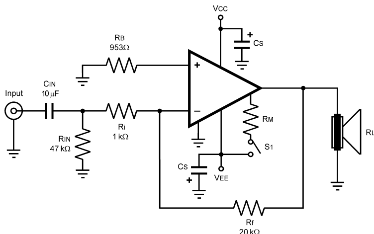
Figure 38. Inverting Amplifier Application Circuit
