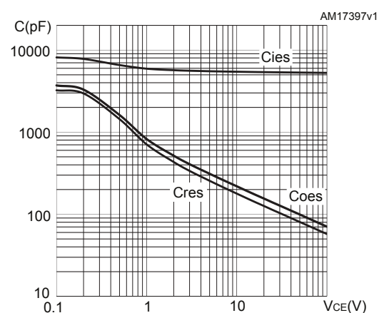
Figure 12. Capacitance variations
