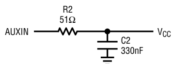
Figure 11. RC Network for V CC Filtering
