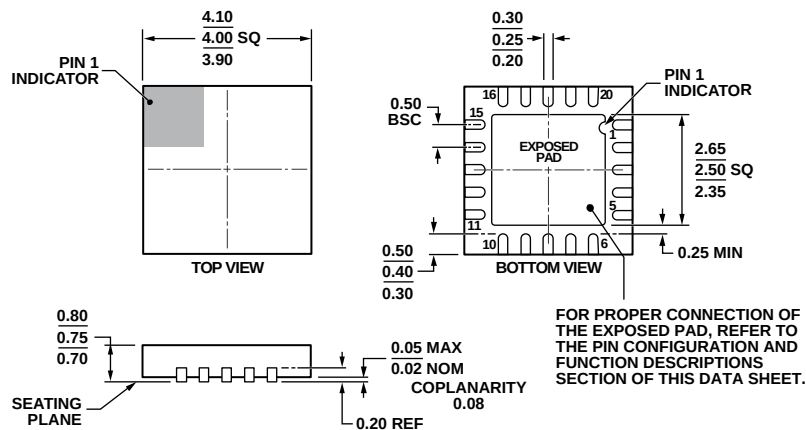
Figure 38. 20-Lead Lead Frame Chip Scale Package [LFCSP] 4 mm × 4 mm Body and 0.75 mm Package Height (CP-20-10) Dimensions shown in millimeters
