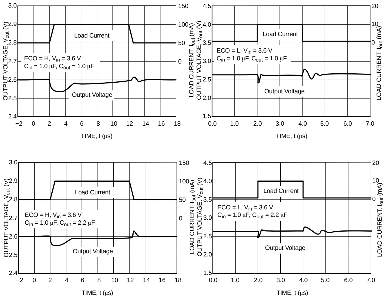
Figure 30. Load Transient Response ( V_{out} = 2.6\text{ V} )
