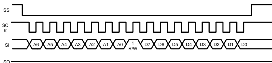
Figure 3. SPI Write Cycle
