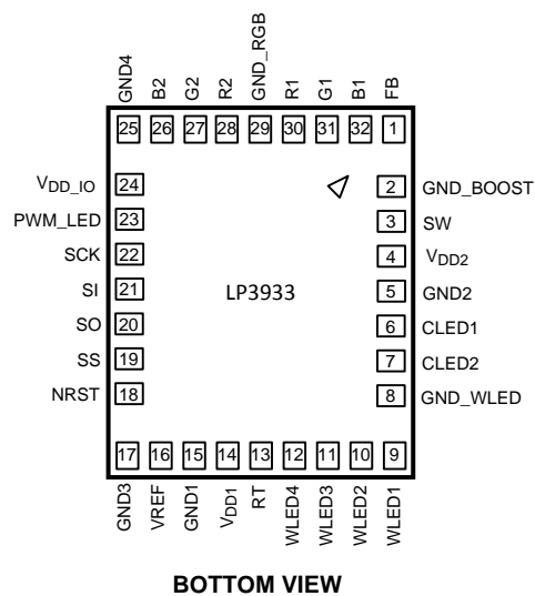
Figure 2. 32-Lead TLGA Package See Package Number NPC0032A
