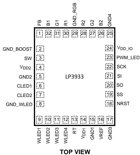
Figure 1. 32-Lead TLGA Package See Package Number NPC0032A
