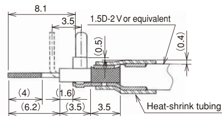
◆Board Termination Pattern
