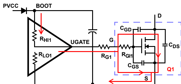
PHASE FIGURE 16. TYPICAL UPPER-GATE DRIVE TURN-ON PATH
