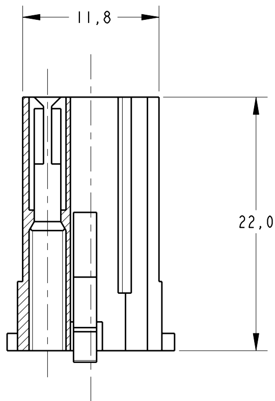
SECTION B-B
