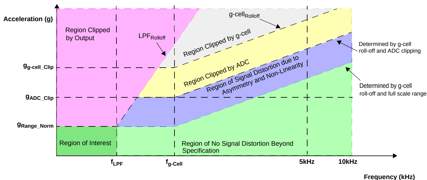
Figure 34. Output Clipping vs. Frequency
