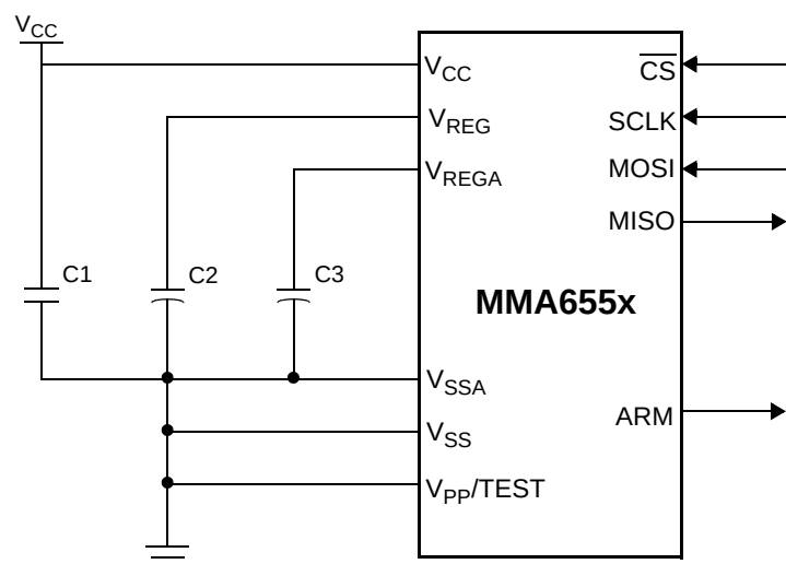
Figure 1. Application Diagram
