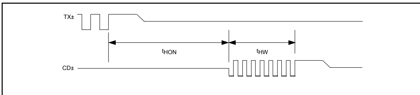
FIGURE 6: Heartbeat Timing
