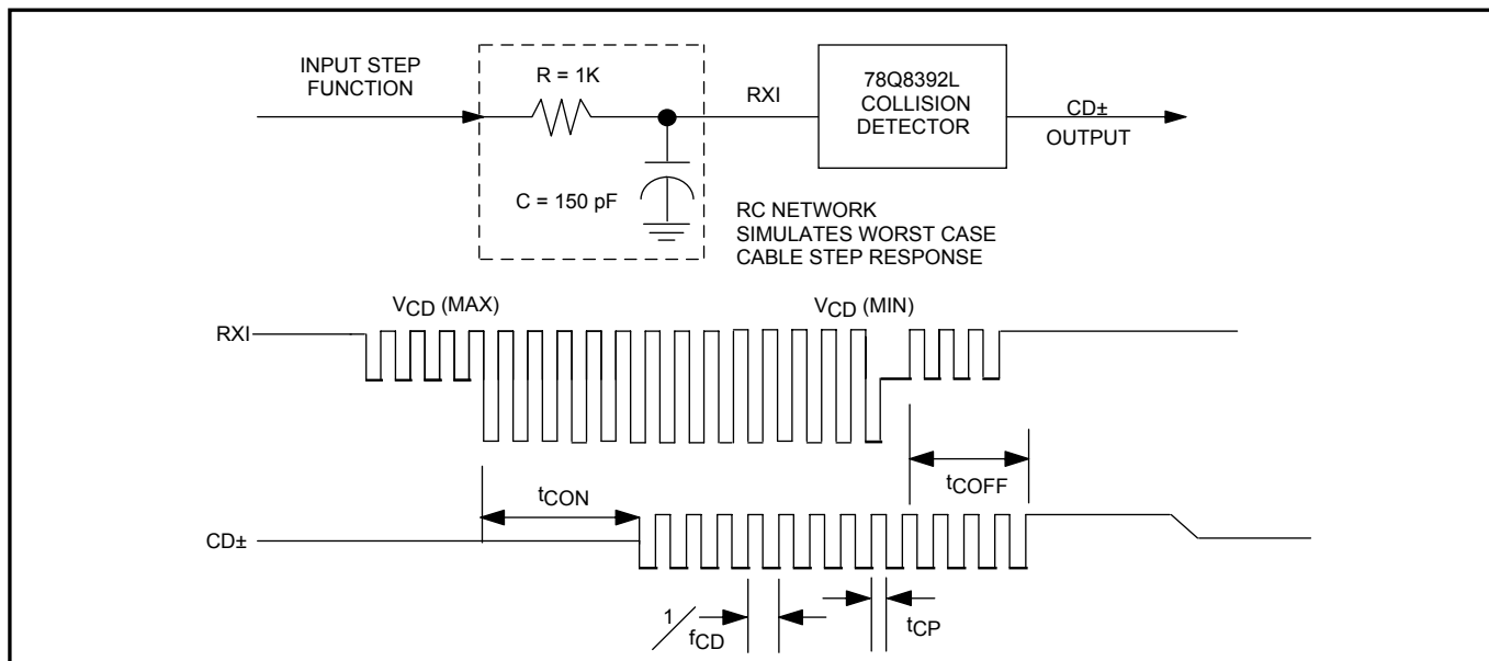
FIGURE 5: Collision Timing
