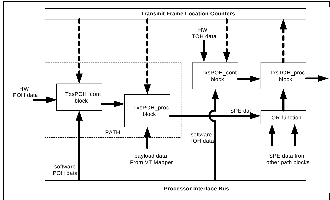
FIGURE 13. SDH TRANSMITTER GENERAL STRUCTURE
