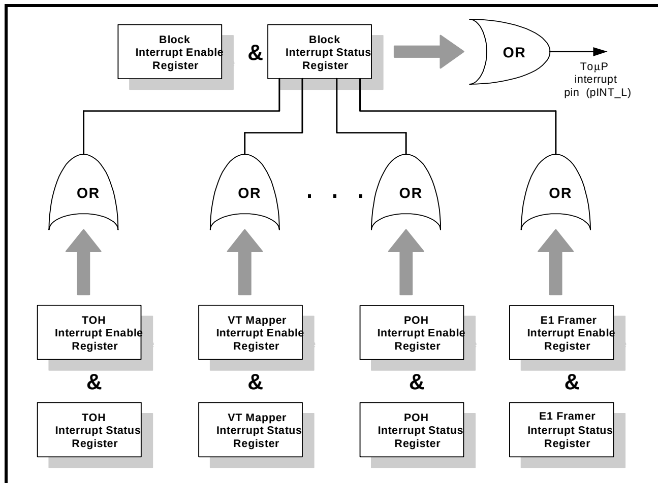
FIGURE 16. INTERRUPT HIERARCHY
