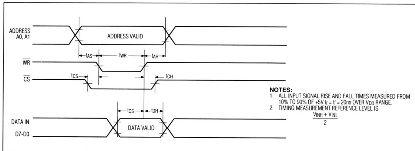
Figure 2. Write-Cycle Timing
