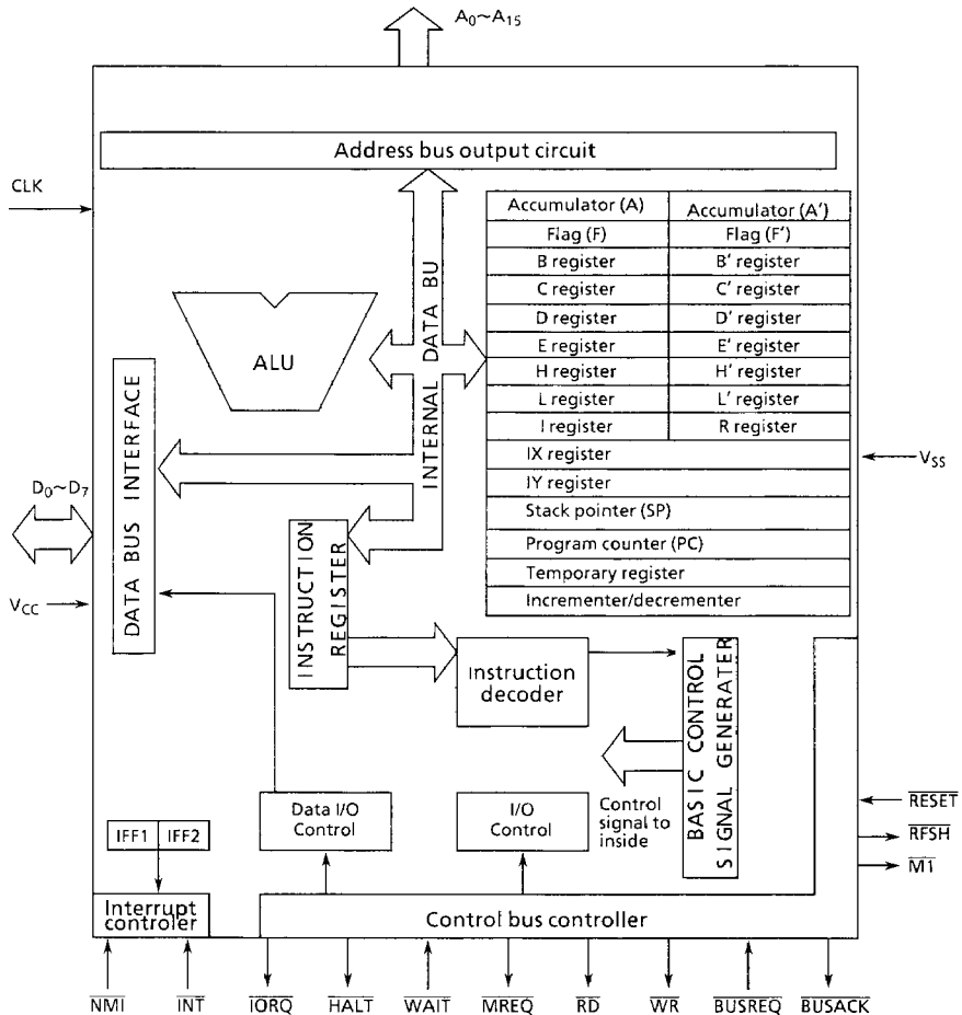
Figure 3.1 Block Diagram
