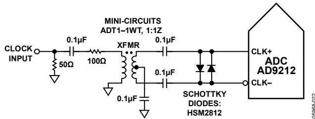
Figure 51. Transformer-Coupled Differential Clock
