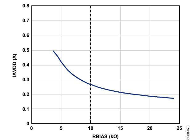
Figure 64. IAVDD vs. RBIAS, AD9212-40
