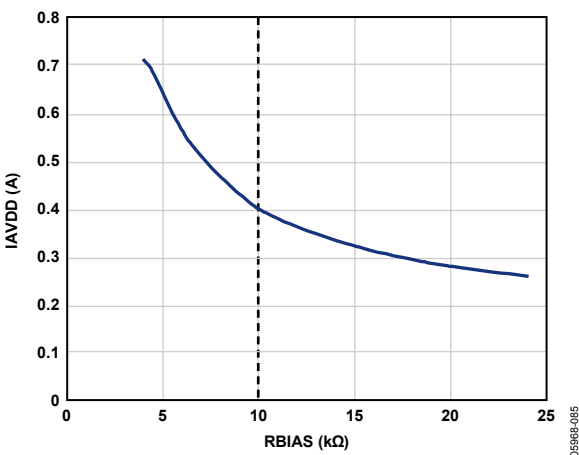
Figure 66. IAVDD vs. RBIAS, AD9212-65
