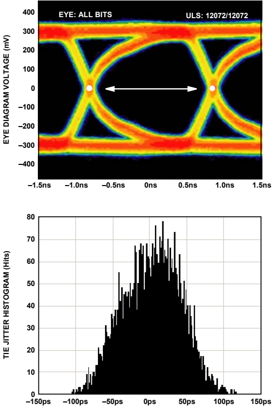
Figure 62. Data Eye for LVDS Outputs in ANSI Mode with 100 \Omega Termination on and Trace Lengths Greater than 24 Inches on Standard FR-4
