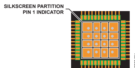
Figure 73. Typical PCB Layout
