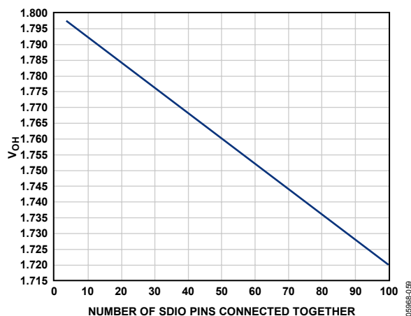
Figure 71. SDIO Pin Loading
