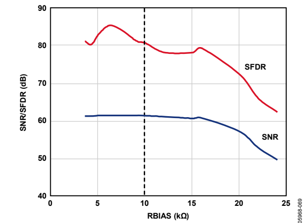
Figure 63. SNR/SFDR vs. RBIAS, AD9212-40
