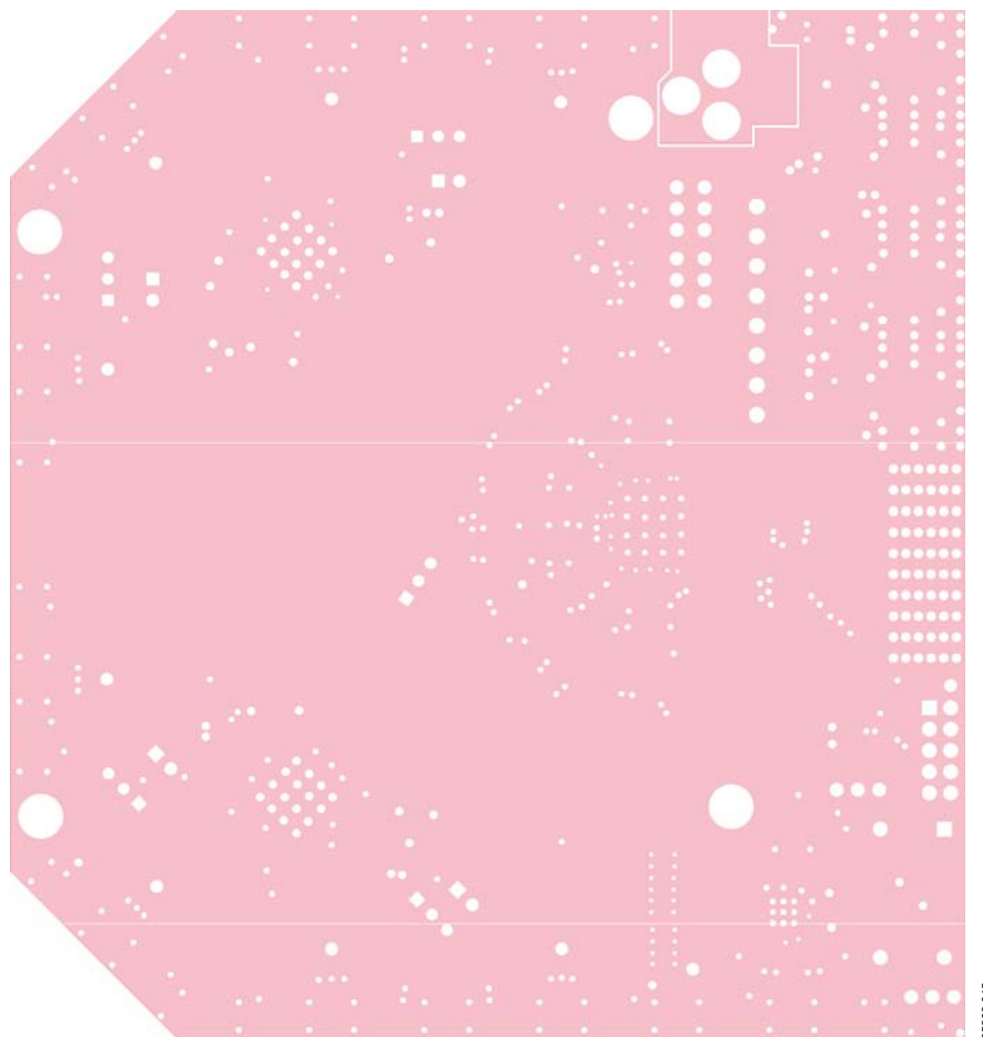
Figure 84. Evaluation Board Layout, Ground Plane
