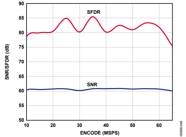
Figure 24. SNR/SFDR vs. f_{\text{SAMPLE}} , f_{\text{IN}} = 35 MHz, AD9212-65
