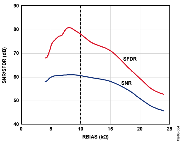
Figure 65. SNR/SFDR vs. RBIAS, AD9212-65
