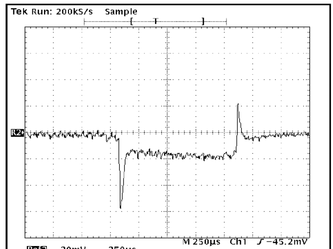
Transient Response Vo=2.8V, Io=300mA to 10A
