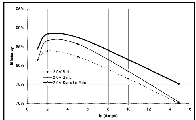
Typical Efficiency at Vo=2.0V
