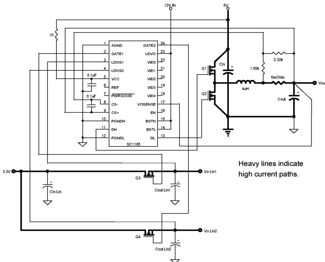
Layout diagram for the SC1185
