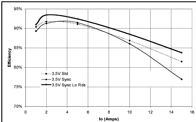
Typical Efficiency at Vo=3.5V
