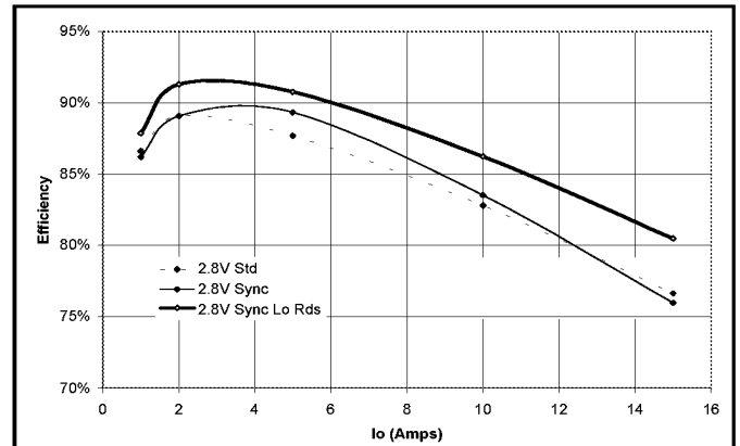
Typical Efficiency at Vo=2.8V
