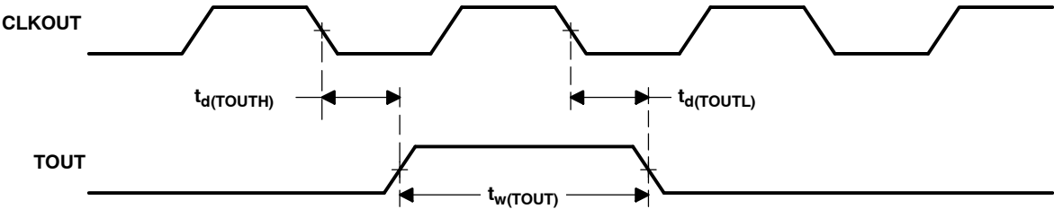
Figure 20. TOUT Timing
