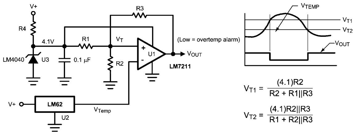
FIGURE 7. Centigrade Thermostat
