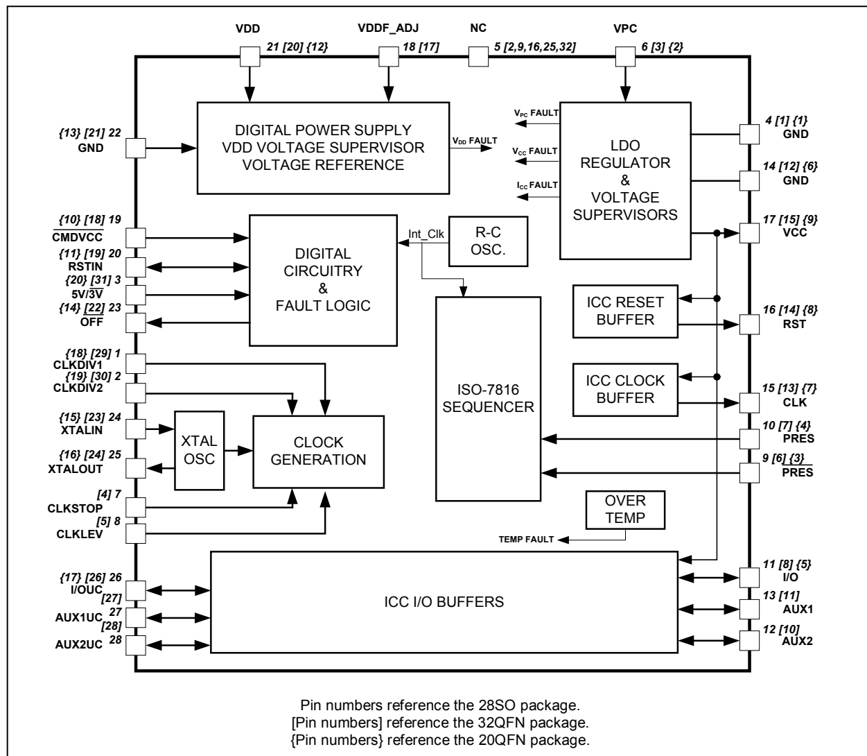
Figure 1: 73S8024RN Block Diagram
