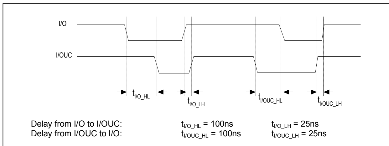
Figure 7: I/O – I/OUC Delays Timing Diagram
