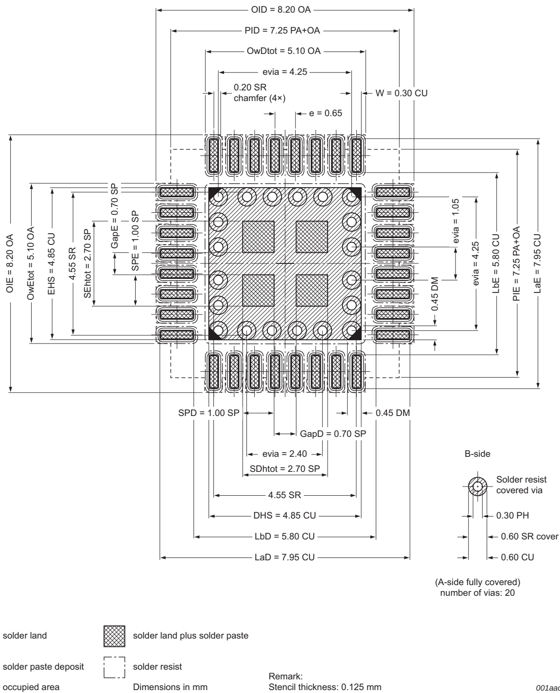
Fig 41. Reflow soldering of the HVQFN33 package
