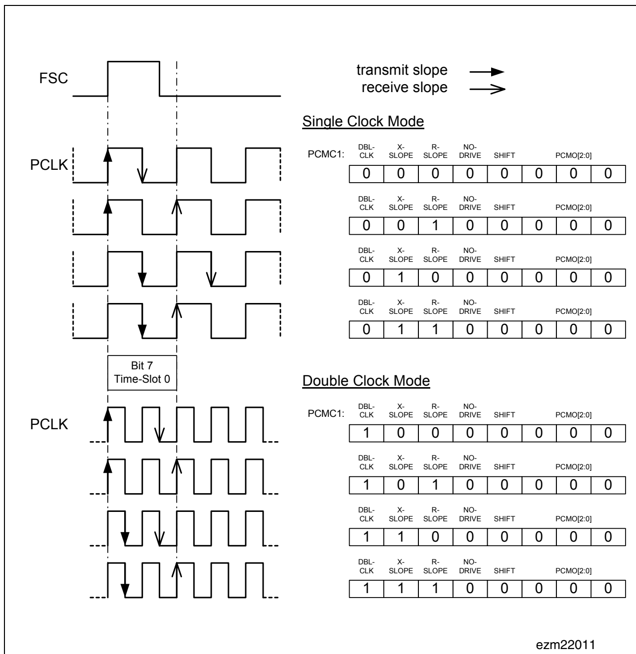
Figure 53 Setting the Slopes in Register PCMC1
