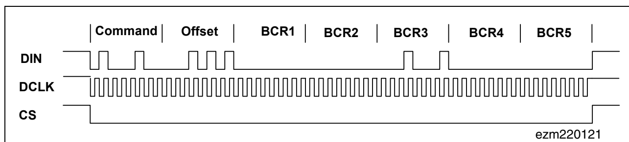
Figure 66 Waveform of Programming Example SOP-Write to Channel 0
