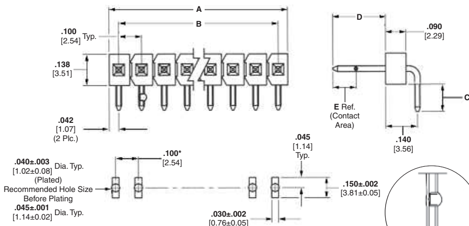
Board Retention using Swaged Tails (All Header Sizes)
