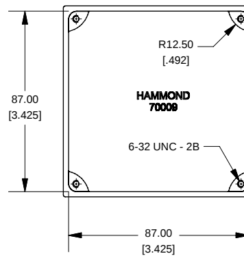
Top View Looking Inside Box
