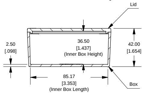
SECTION B-B Side View of Assembly
