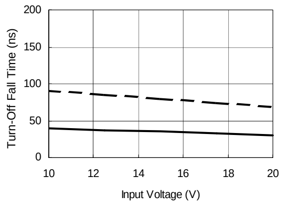
Figure 7B. Turn-Off Fall Time vs. Input voltage
