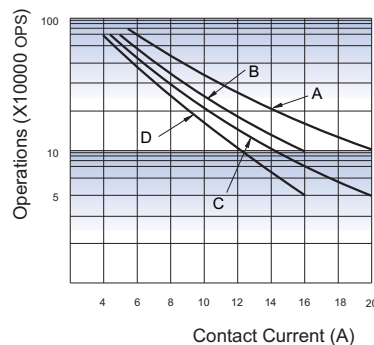
ENDURANCE CURVE
